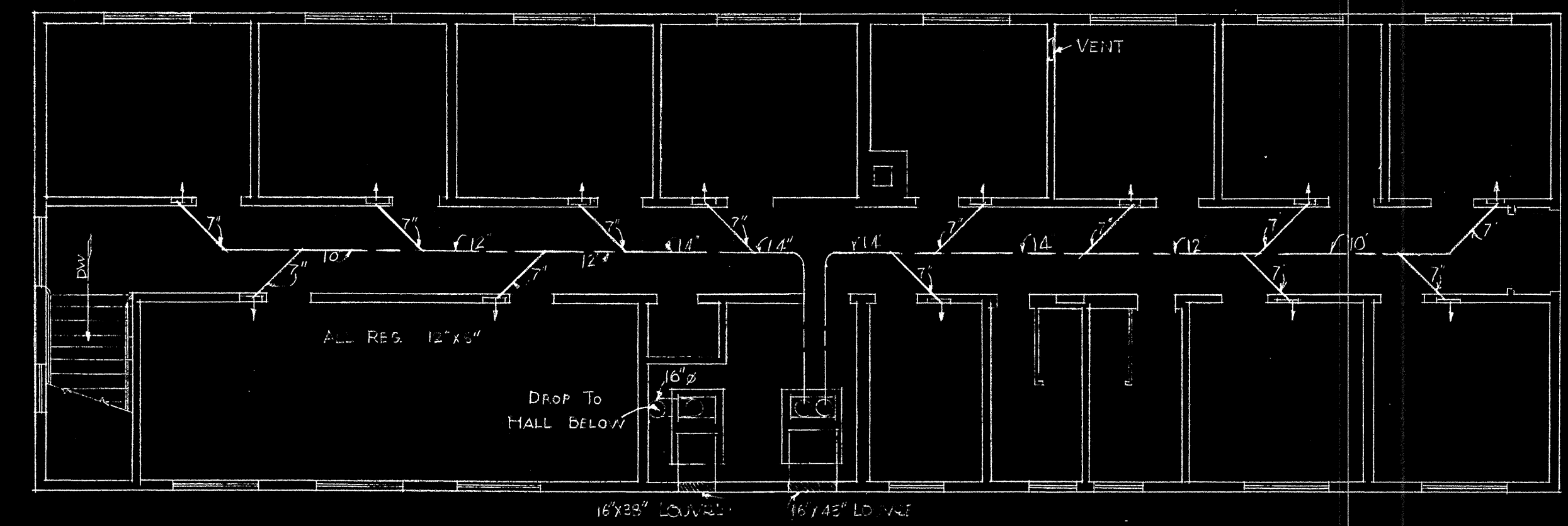
SECOND FLOOR PLAN SCALE \frac{1}{8}" = 1'-0"
